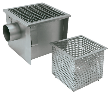
Sumidero 250x250mm
